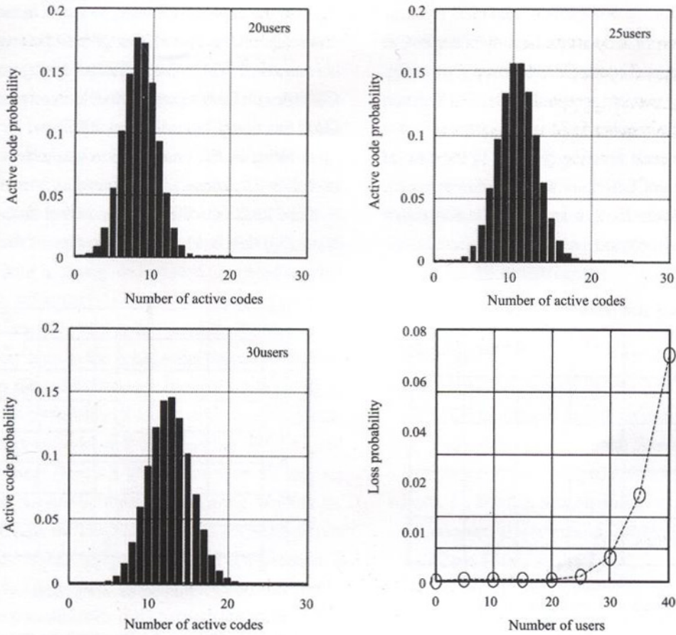
Fig. 4. Distribution of the voice users and Loss probability in classical CDMA.
