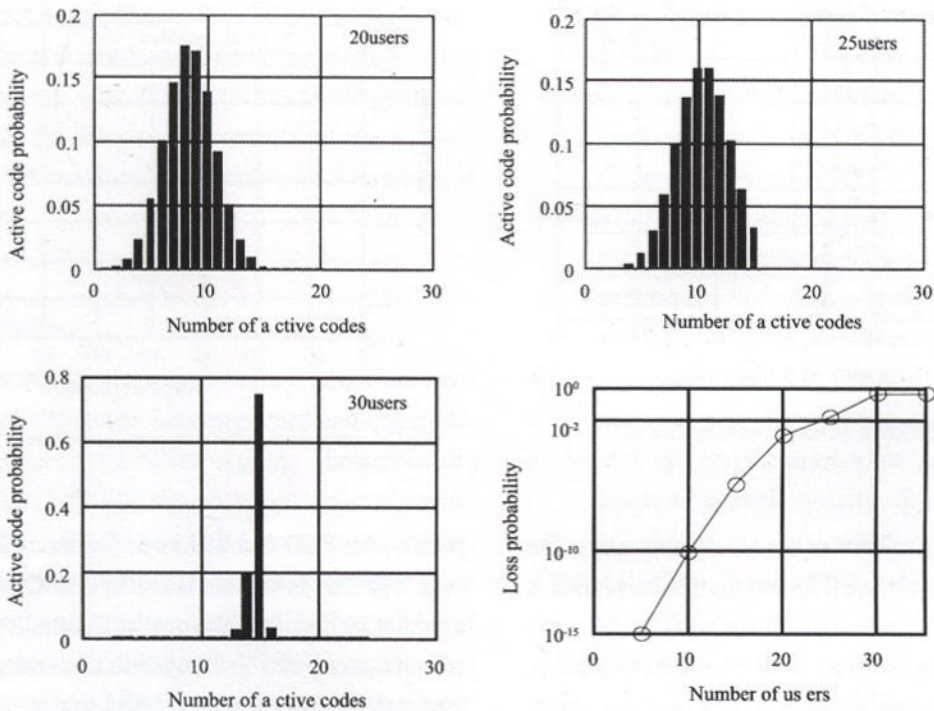
Fig. 5. Distribution of the voice users and Loss probability
