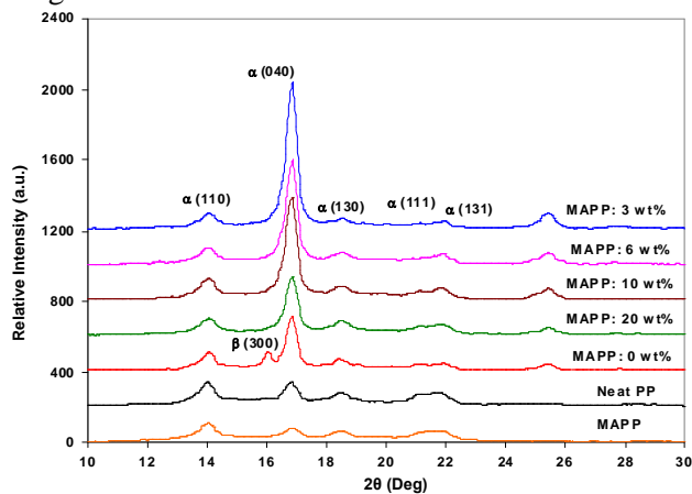
Fig.3 WAXRD patterns of neat PP, MAPP and 5 wt% filled PP/clay nanocomposites.
