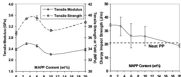
Fig.2 Mechanical properties of 5 wt% filled PP/clay nanocomposites.
