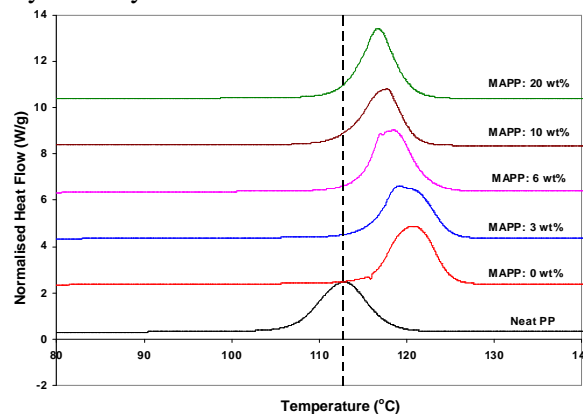
Fig.4 DSC curves of neat PP and 5 wt% filled PP/clay nanocomposites at a cooling scan.
