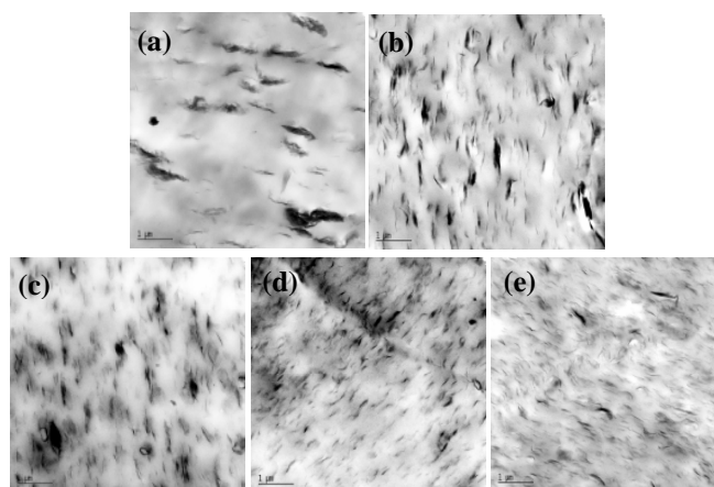
Fig.1 TEM micrographs of 5 wt% filled PP/clay nanocomposites at 15000 \times magnification with various MAPP contents: (a) 0 wt%, (b) 3 wt%, (c) 6 wt%, (d) 10 wt% and (e) 20 wt%.
